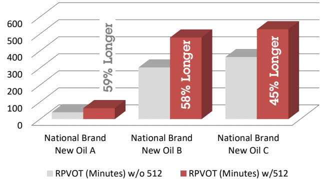
Oxidative Life of Three National Brand Hydraulic Oils With & Without SWEPCO 512
